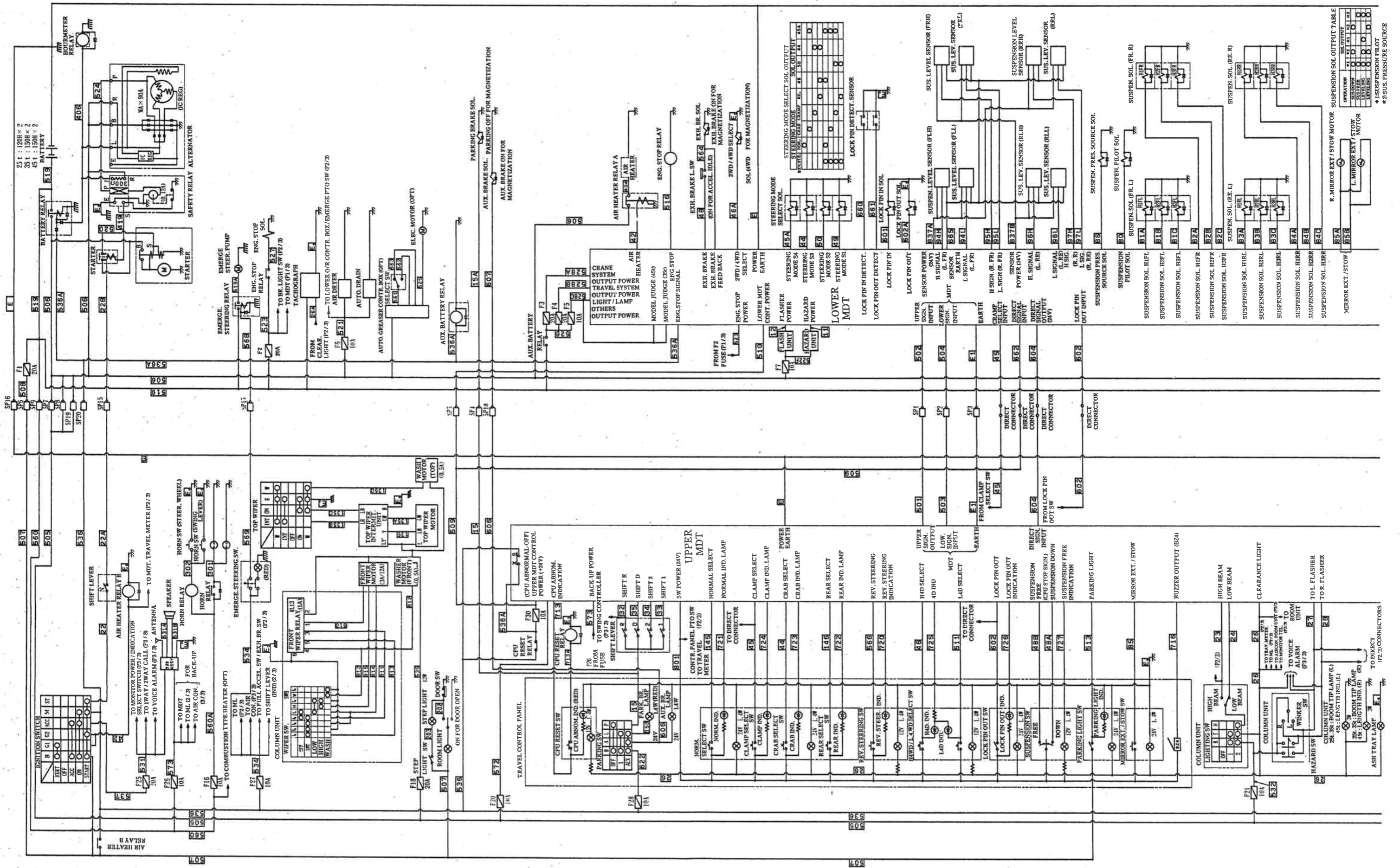
Fig. 1-2 General Wiring Schematic (1/3)
